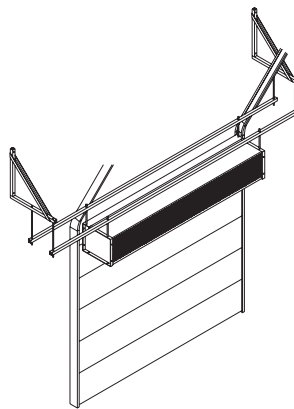
Wall Mount Brackets w/Threaded Rod & Strut for Door Track Clearance
