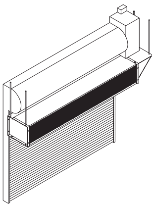
Ceiling Mount w/Extension Bracket for Operator Clearance
