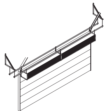
Tandem Unit Mount
