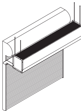
Ceiling Mount w/Custom Air Discharge Nozzle
